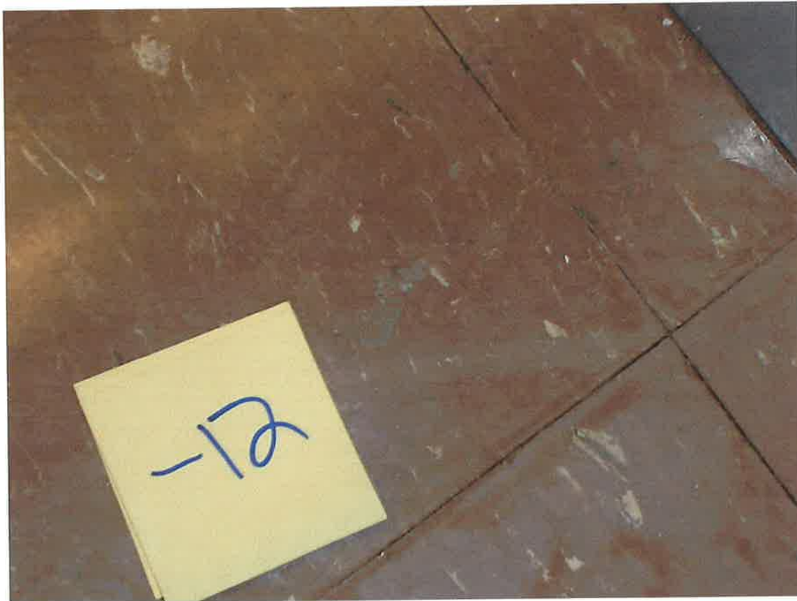
HA #12 – Asbestos containing 12” x 12” dark brown floor tile with cream and green streaks and non asbestos containing associated mastic
