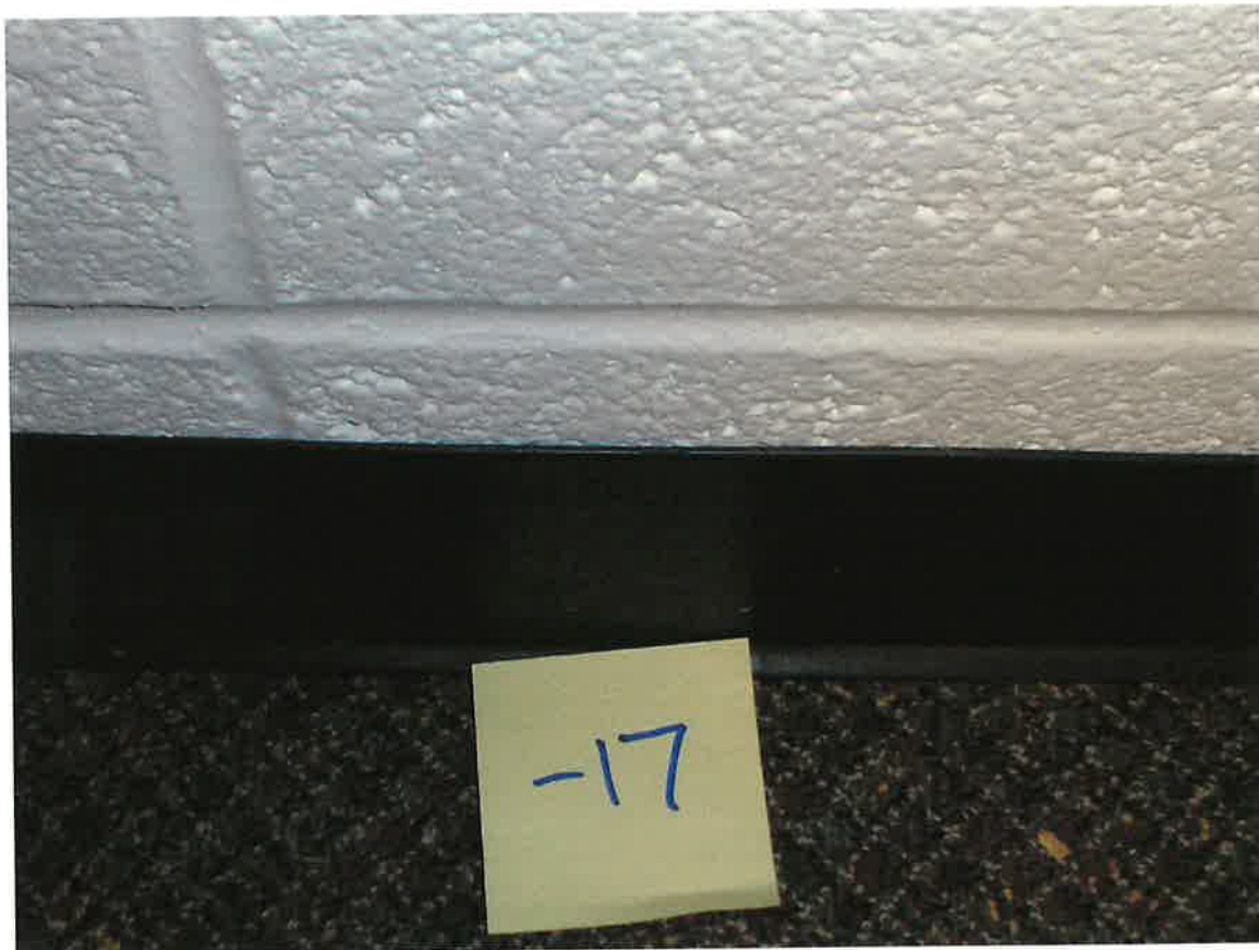
HA #17 – Non asbestos containing 4” black cove molding and associated mastic
